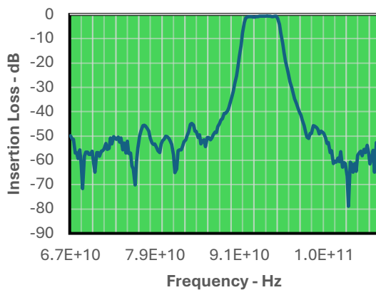
Full Band Filter Response S21
